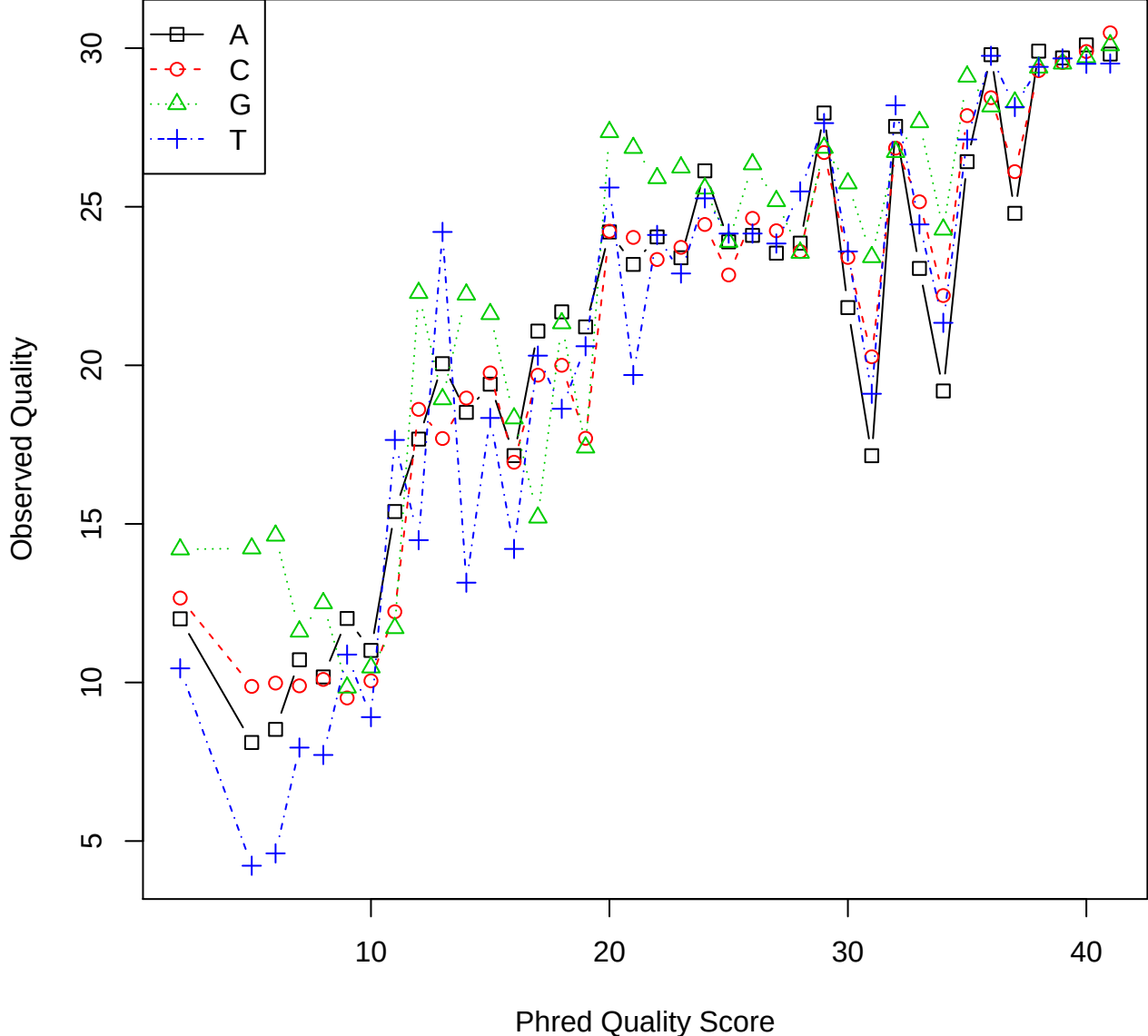
Observed Quality vs. Phred Quality Score
